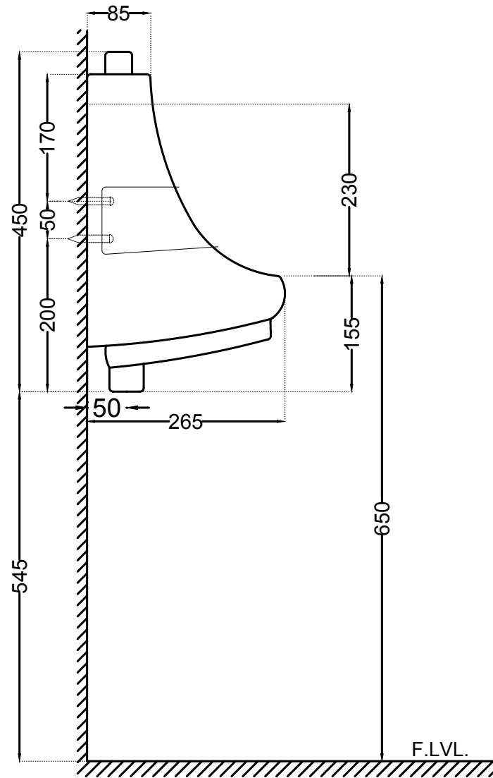
SIDE VIEW
